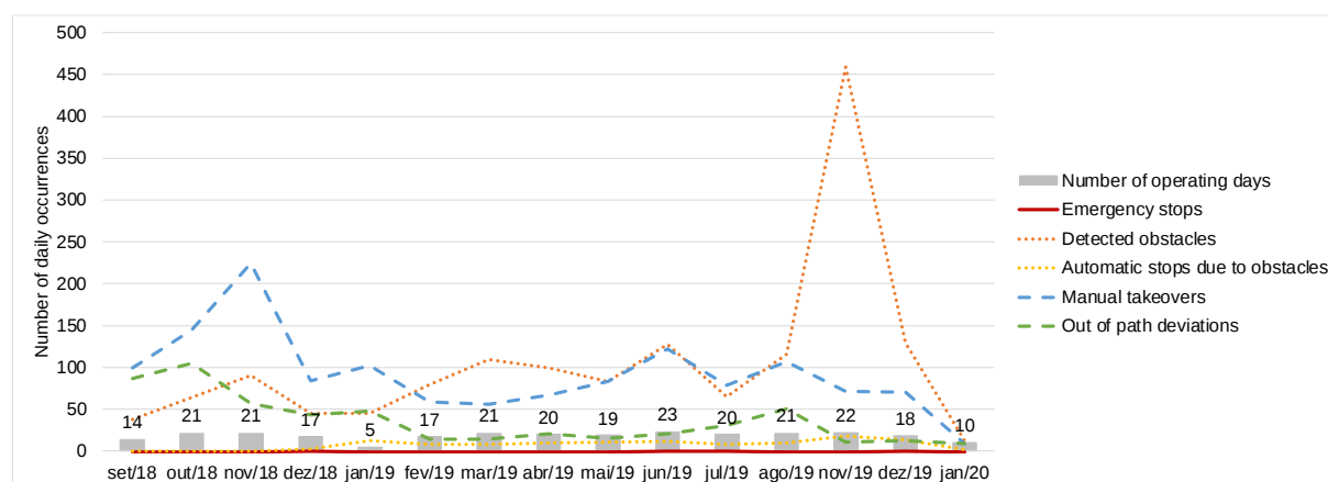
Figure 9. Pfaffenthal shuttle performance overtime Source: prepared by the authors based on Navya's data
